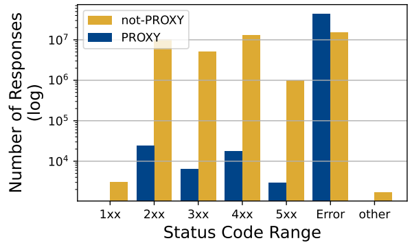
(b) HTTPS
