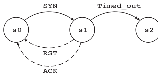
Figure 9: Half-Open TCP state transition diagram.
