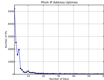
Figure 4: Phishing uptime between 0-60 days.
